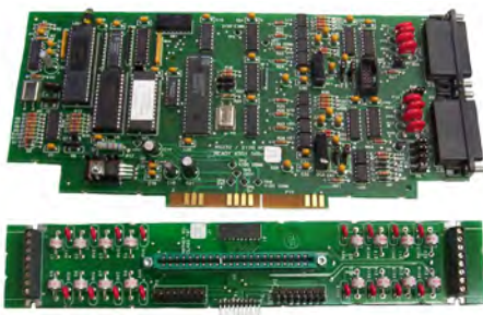
4100-0154K Motherboard (lower – fitted to the 4100ES FIP) and Interface Module (upper – fitted into the Motherboard))
