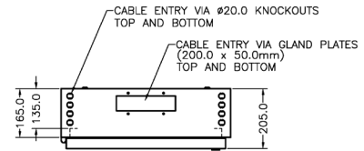
Top View - 135 Deep Cabinet
