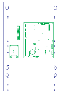
MX4428 Main Board Mounting
