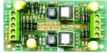
PA0646 ALIM9706 Audio Line Isolator Module
