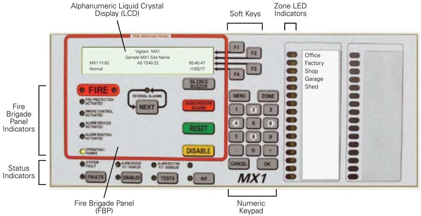
Fig 1-1 Operator Interface
