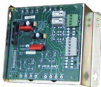
FP1076 TRAN9705-4 (PA0794) 2x25W Transformer Module c/w Relays incl. PA0650 EAMP9001
