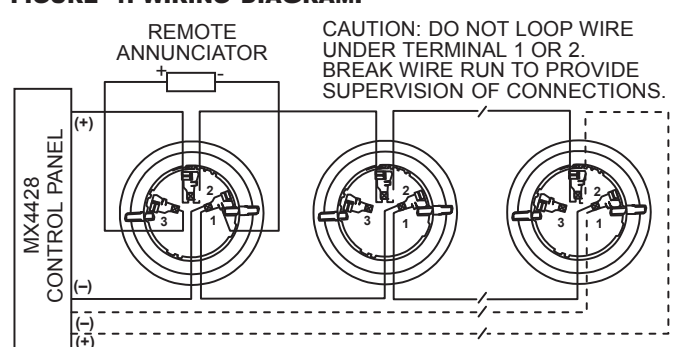
FIGURE 1. WIRING DIAGRAM:
