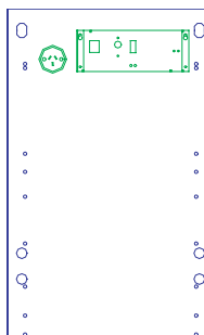
MX4428 6A PSU Brick Mounting
