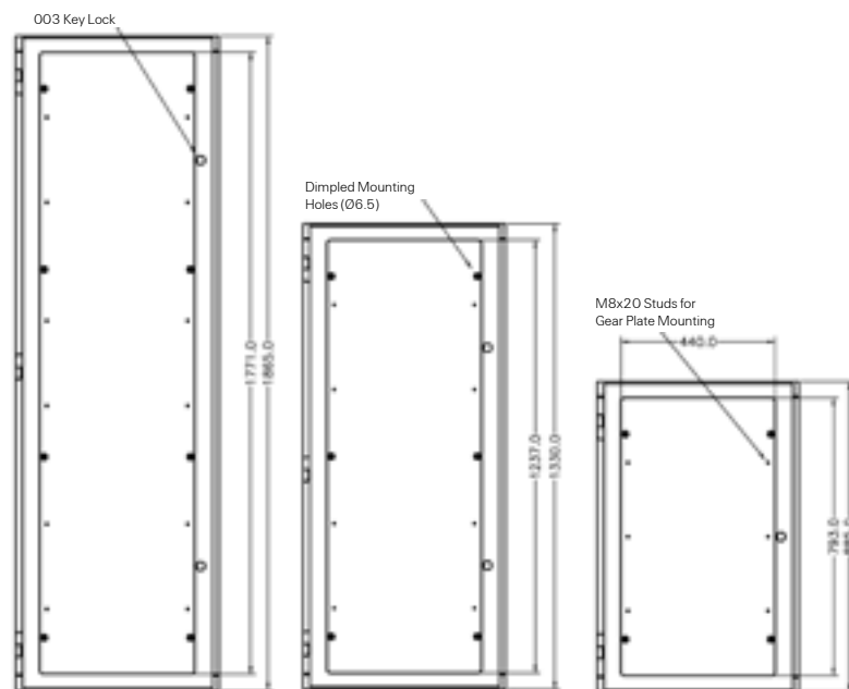
40U Cabinet
