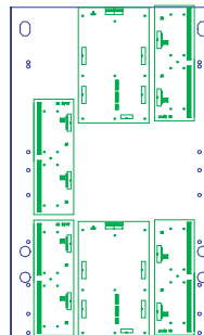
IOR & Termination Board Mounting
