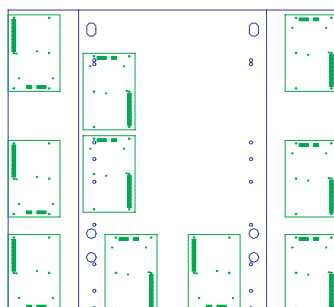
ADR/MPR Mounting
