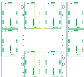
IOR Mounting
